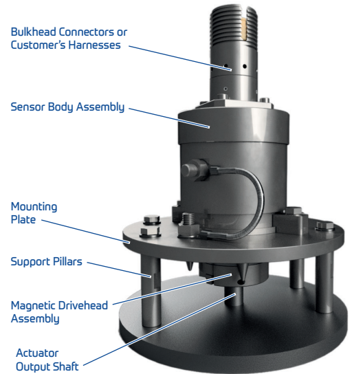
PM1 Pillar Mounted Single Output
