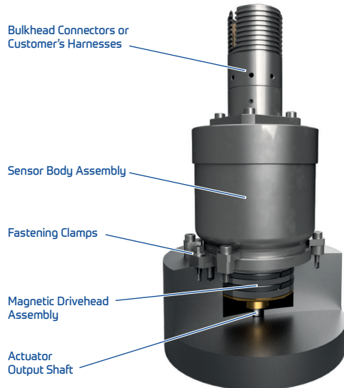
FF1 Flush Fitting Single Output
