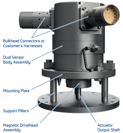
PM2 Pillar Mounted Dual Output
