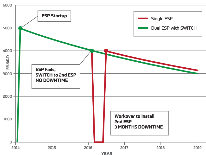
Continual Production with SWITCH v Workover and Deferred Production due to Pump Failure
